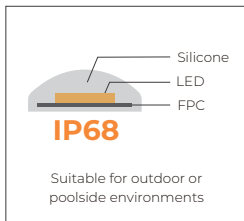
Solid dome co-extrusion
